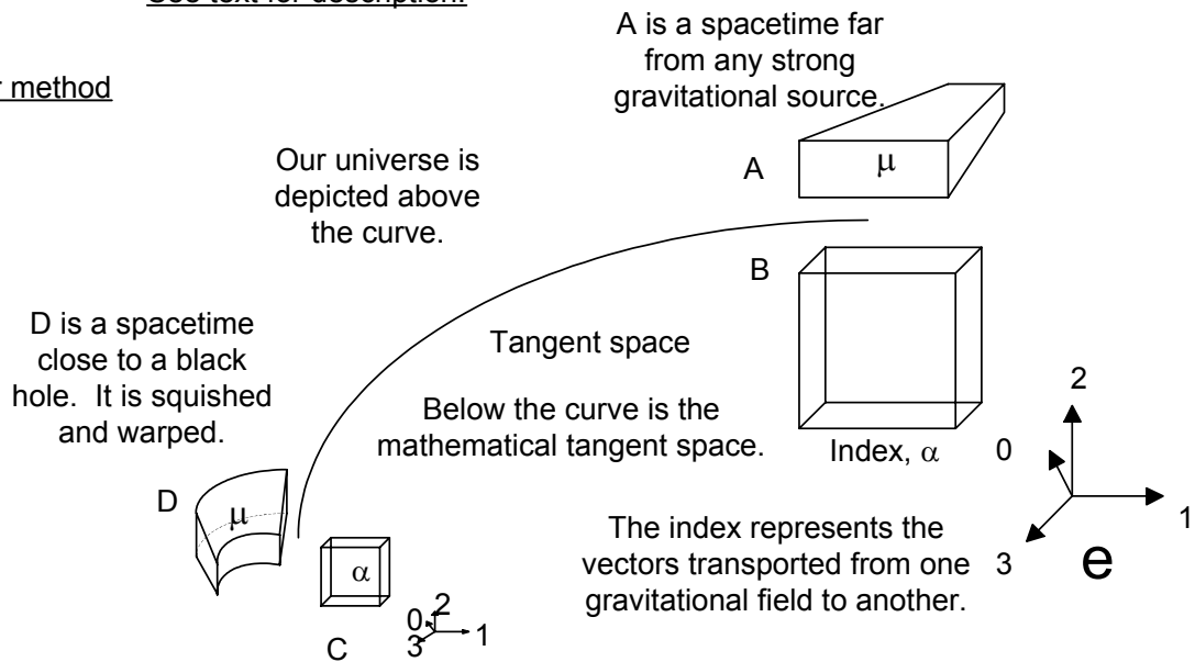
Figure 2-10 Tetrad and Tensors See text for description.
