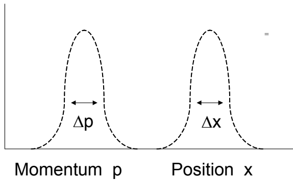
Figure 10-1 Heisenberg Uncertainty
