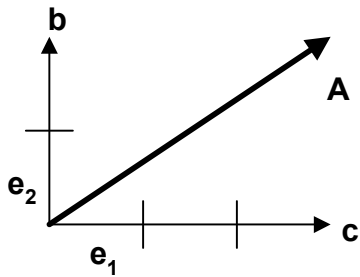
Figure 1-6 Vectors
