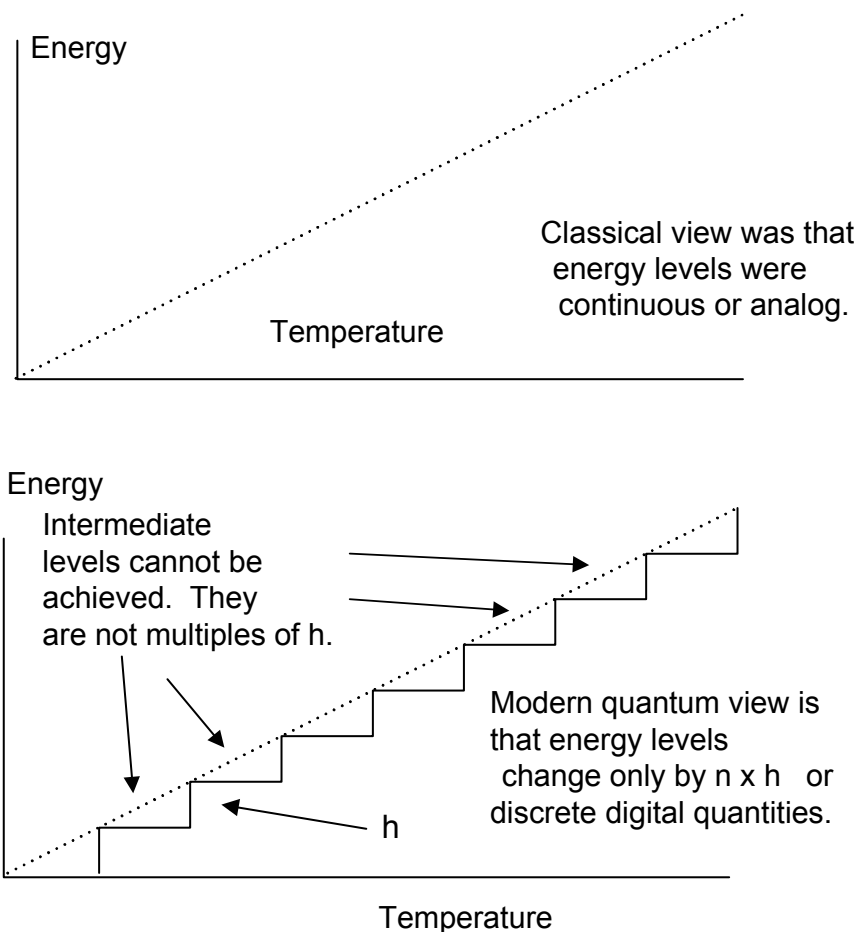
Figure 3-4 Quantum Postulate
