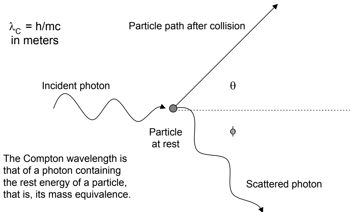
Figure 5-8 Compton Wavelength
