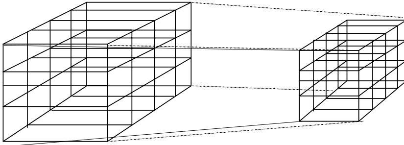
Figure 6-3 The result of using the wedge product is an egg crate or tubes in spacetime that define magnetic field lines.
