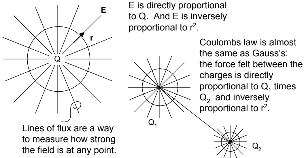
Figure 5-2 Gauss's Law for Electric Charge
