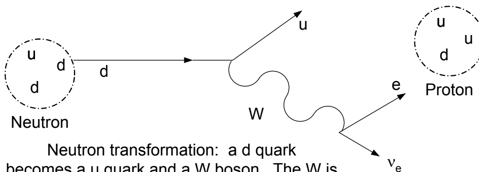
Figure 12-1 Electroweak Theory
