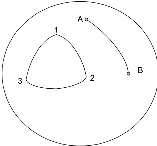
Figure 4-1 Curved Space
