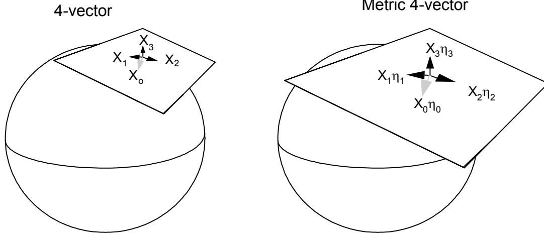
Figure 2-11 Metric Vectors
