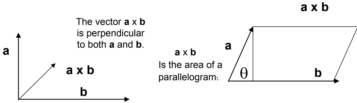
Figure 4-5 Cross Product
