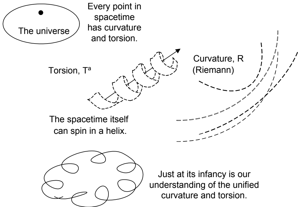
Figure I-2 Evans Spacetime
