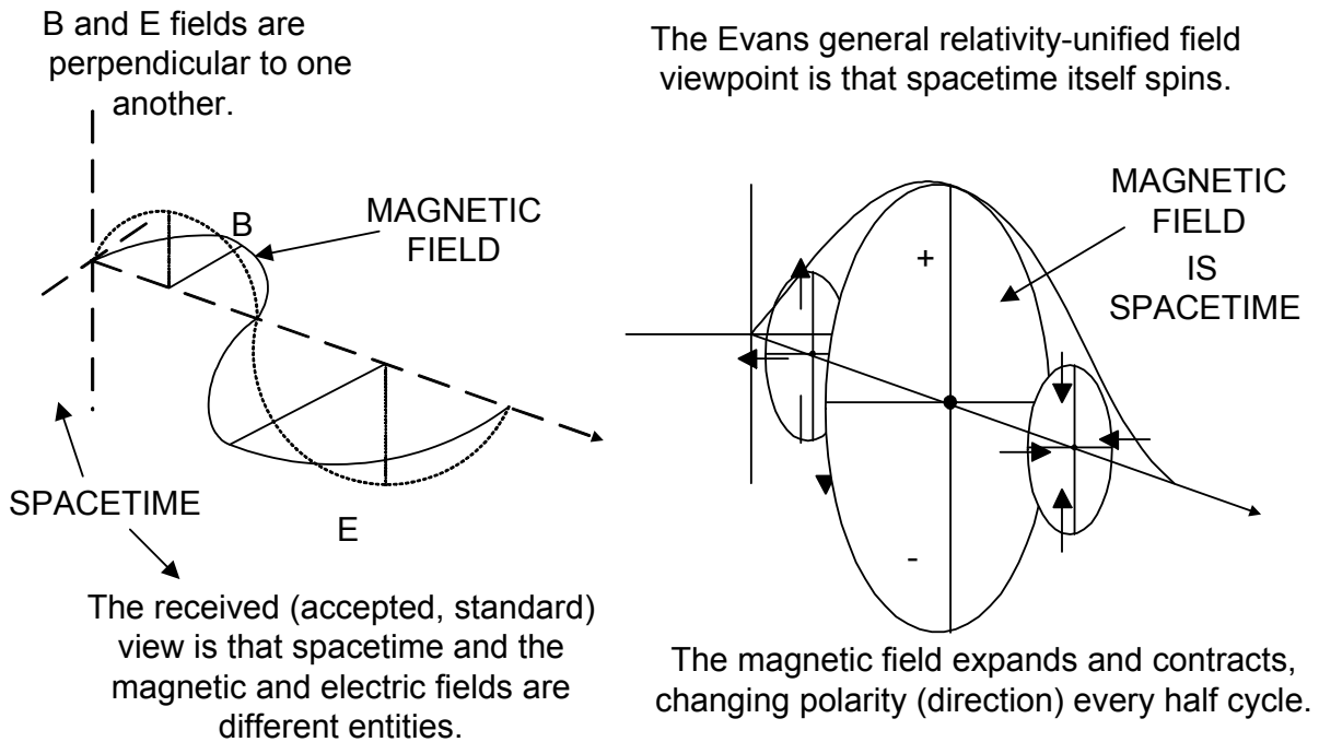
Figure 11-1 Depiction of the Magnetic and Electric Fields
