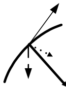
Figure 8-8 (\square + kT) q^a_{\mu} = 0
