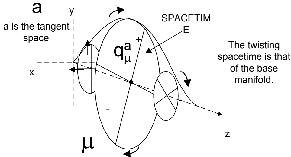
Figure 8-7 The magnetic field is spinning spacetime.
