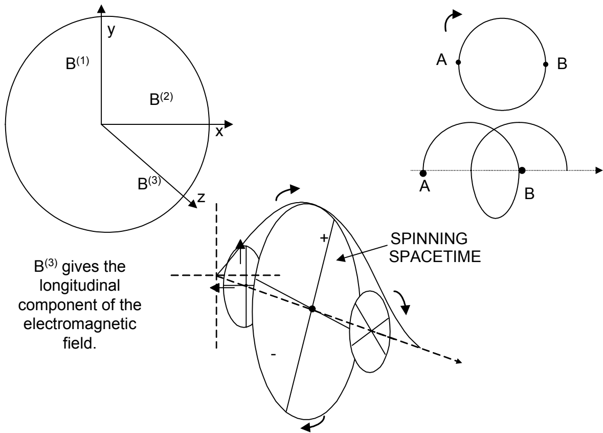
Figure 11-4 Basic Geometry
