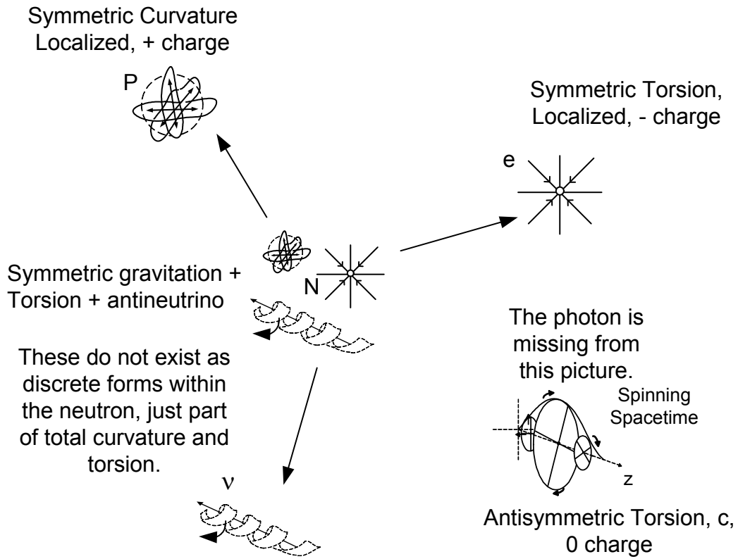
Figure 15-4 Enigmatic Neutron
