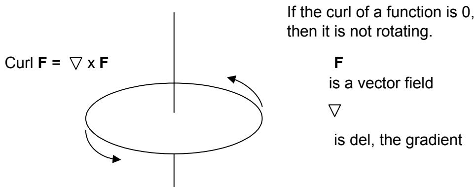
Figure 4-7 Curl
