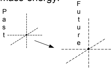
Figure 2-5 Stress Energy =
